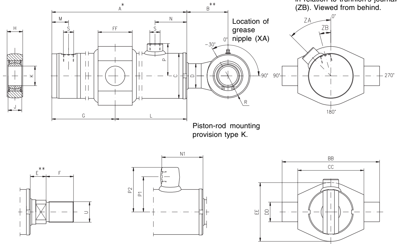
Piston-rod mounting provision type U. N.B. Dimensions as on page 4.
